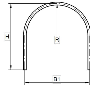
U-Bogen
